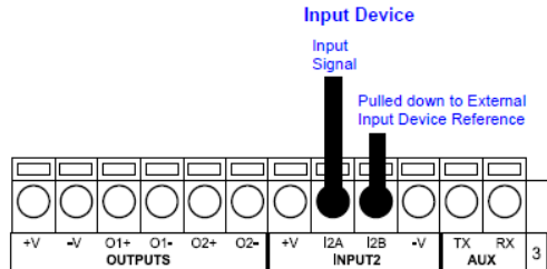
Figure 17 - PNP Input 2 Using External Power
