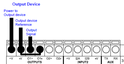
Figure 20 - Open Collector Output Using CBX
