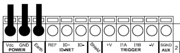
Power to External Illuminator
